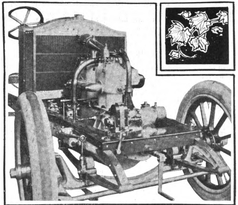
Figure III—Thirty—Special—Motor, Magneto, and Thermo-Syphon Cooling
